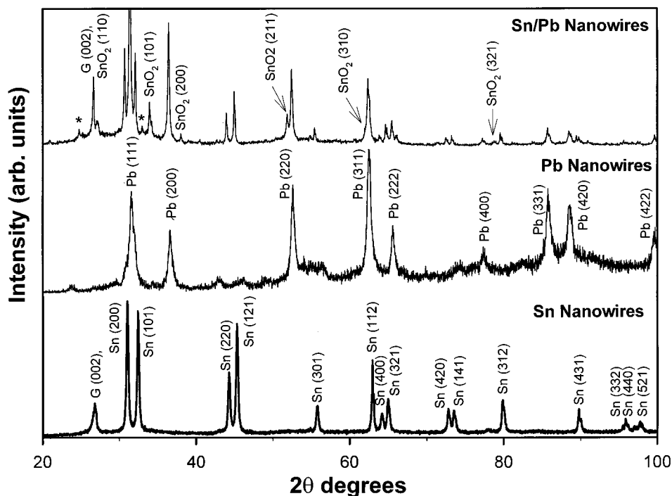
Figure 3. X-ray diffraction of Sn–Pb nanowires (top) compared with Pb nanowires (middle) and Sn nanowires (bottom). The \text{SnO}_2 reflections (denoted by arrows) arise from residual unreacted Sn, and the minor star peaks cannot be identified. (EDX analyses showed that oxygen is absent from the nanowires). Compared with a single metal (Pb or Sn), the lattice parameter for Pb–Sn nanowires remained unchanged.
