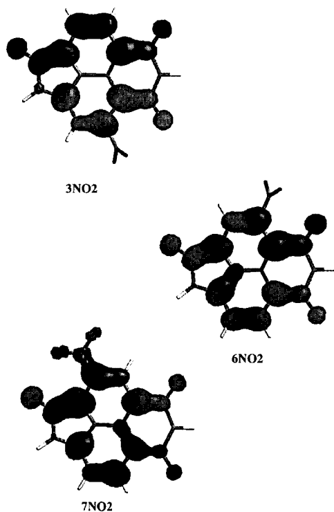
Figure 2. B3LYP/6-31G(d) optimized geometries and LUMO of 3NO2 , 6NO2 and 7NO2 molecules
