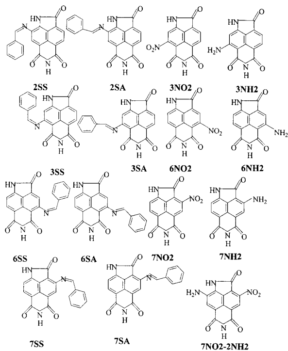
Figure 1. Structures of the substituted lactamimides studied
