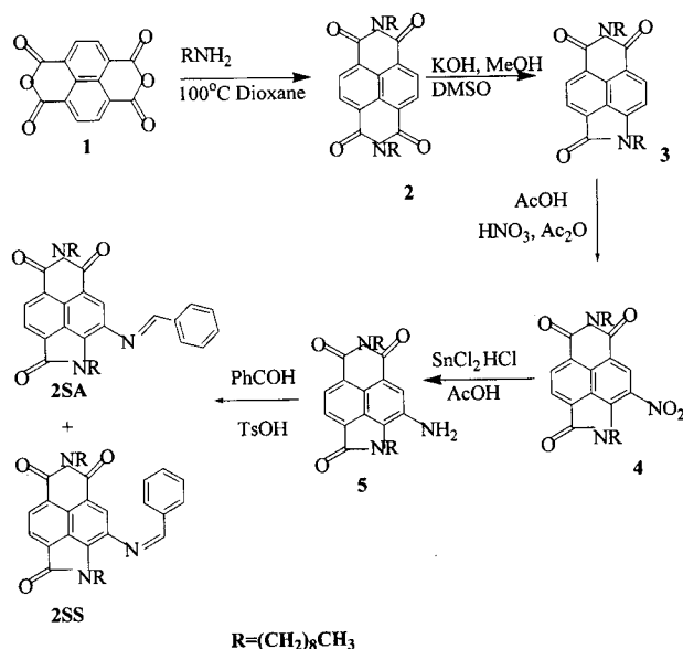
Scheme 1. Synthetic route to 2-substituted lactamimides
