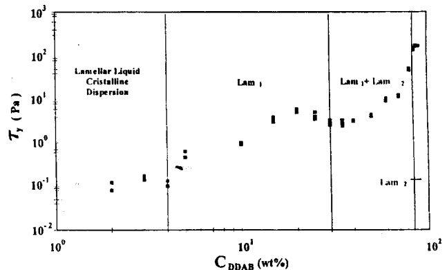
Fig. 6 Yield stress as a function of DDAB concentration
