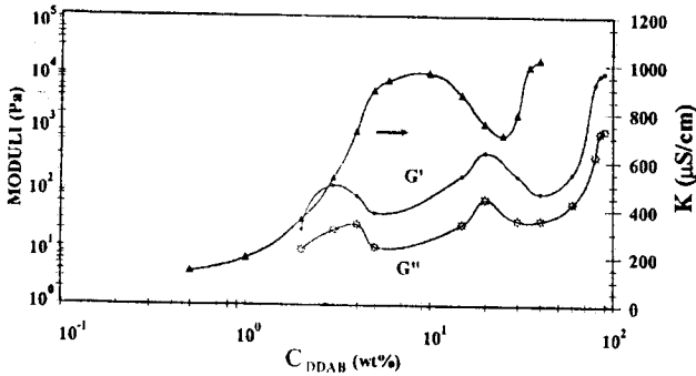
Fig. 8 Elastic (●) and viscous (○) moduli and electrical conductivity (▲) as a function of DDAB concentration
