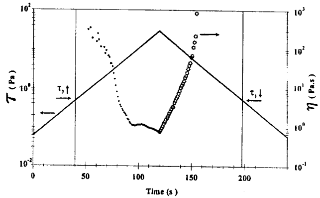
Fig. 10 Applied stress and shear viscosity as a function of time in an exponentially increasing and decreasing stress program applied to a 10 wt% DDAB sample
