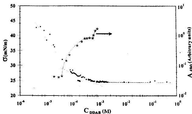
Fig. 1 Surface tension and Sudan III solubilization absorbance, measured at 490 nm, versus didodecyltrimethylammonium bromide (DDAB) concentration
