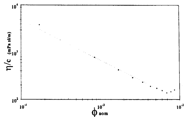
Fig. 4 Relative viscosity as a function of nominal volume fraction
