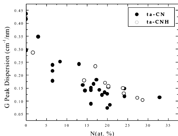
Fig. 11. G peak dispersion for both ta-C:N and ta-C:H:N samples at increasing nitrogen content. The y-axis is the slope (in \text{cm}^{-1}/\text{nm} ) of the linear fit to the G position vs. the three excitation wavelengths for the samples shown in Fig. 6. Similarly, the G dispersion was calculated for the remaining nitrogen content films, not shown in Fig. 6.
