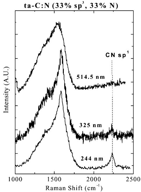
Fig. 4. Raman spectra of a ta-C:N sample measured at different excitation wavelengths. Notice how the 'shape' of the spectra changes with the laser wavelength. CN–sp 1 bonds are remarkably enhanced for UV–Raman.
