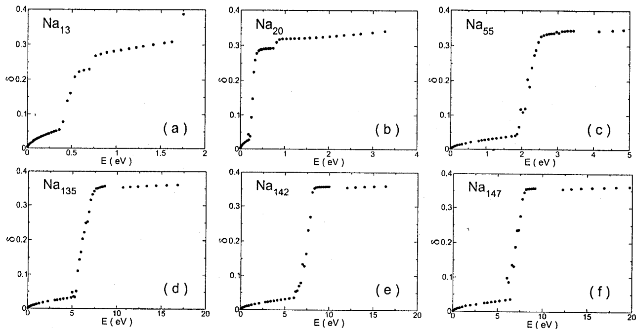
FIGURE 4. RMS bond-length fluctuations of \text{Na}_N , N = 13 (a); 20 (b); 55 (c); 135 (d); 142 (e); and 147 (f); clusters. The cluster energy is calculated taking as reference the value of the binding energy of the most-stable (lowest-energy) configuration given in Table I.
