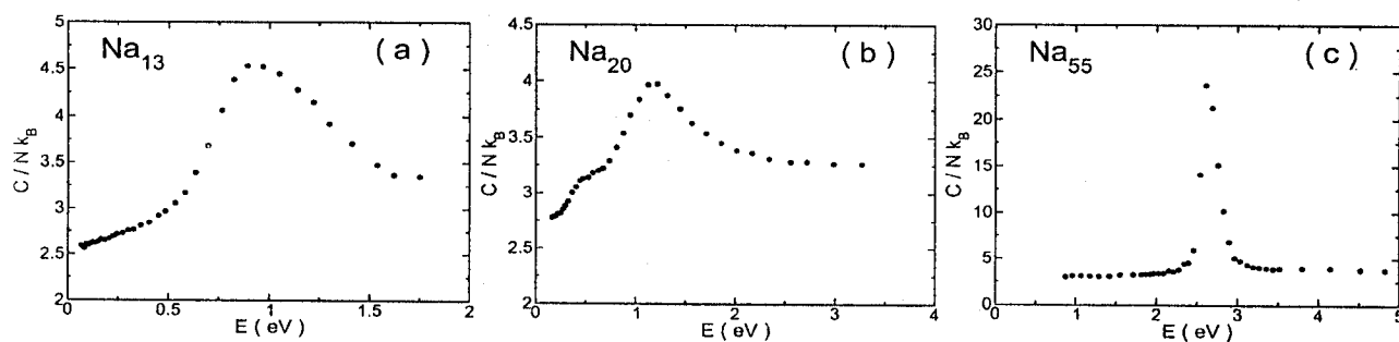
FIGURE 3. Specific heats of \text{Na}_N , N = 13 (a); 20 (b); and 55 (c); clusters. The cluster energy is calculated taking as reference the value of the binding energy of the most-stable (lowest-energy) configuration given in Table I.
