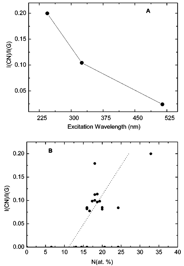
FIG. 22. (a) Variation of CN peak to G peak intensity ratio I(\text{CN})/I(\text{G}) with excitation wavelength for the sample of Fig. 16. (b) Variation of I(\text{CN})/I(\text{G}) with N content, measured at 244 nm; the dotted line is a guide to the eye.
