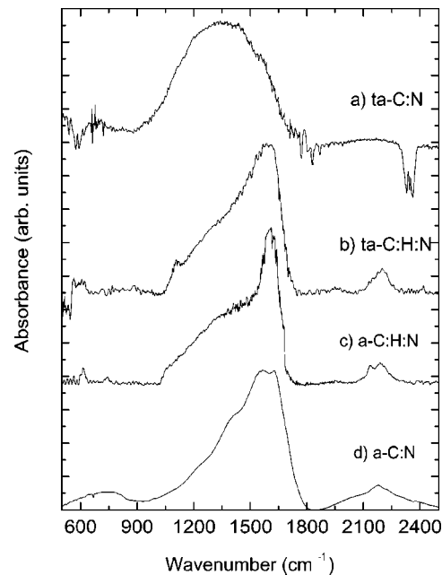
FIG. 9. Comparison of IR spectrum of the four classes of carbon nitrides, (a) ta -C:N, 23 % at. N (b) ta -C:H:N, 28.7 at. % N, 26 % at. H, (c) a -C:H:N, 20% at. N, 35 % at. H (estimated values) (d) a -C:N, 31% N.
