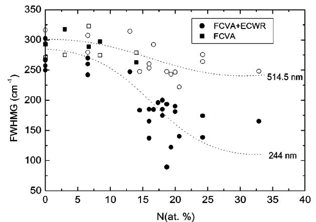
FIG. 18. Variation of G peak FWHM with N content for ( t ) a -C:N films. Circles represent samples deposited by FCVA+ECWR and squares samples deposited by FCVA only. Open symbols refer to 514.5 nm excitation, full symbols refer to 244 nm excitation. The lines are guides to the eye.
