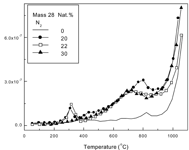
Fig. 5. Effusion transients of nitrogen (mass 28) for ta-CHN films of different nitrogen content. The vertical axis is the quadruple mass analyzer signal normalized to the studied volume and the calibration factor for N_2 .
