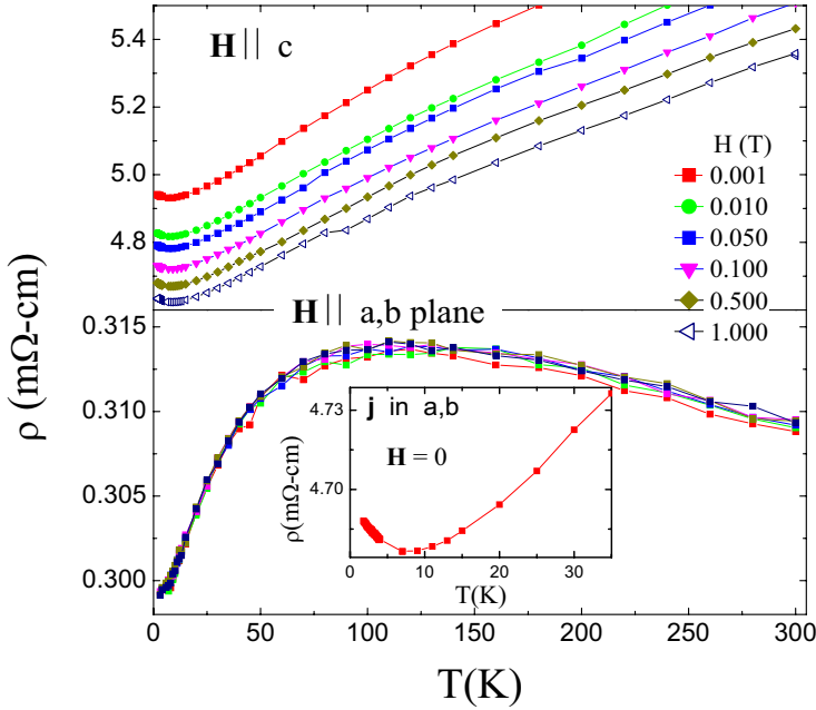
Fig. 3. \rho(T) dependence with applied magnetic fields. The current is in a , b plane and c direction, H is perpendicular to them. The inset shows the curves for H = 0 . Note the minimum below 10 K attributed to a Kondo anomaly.
