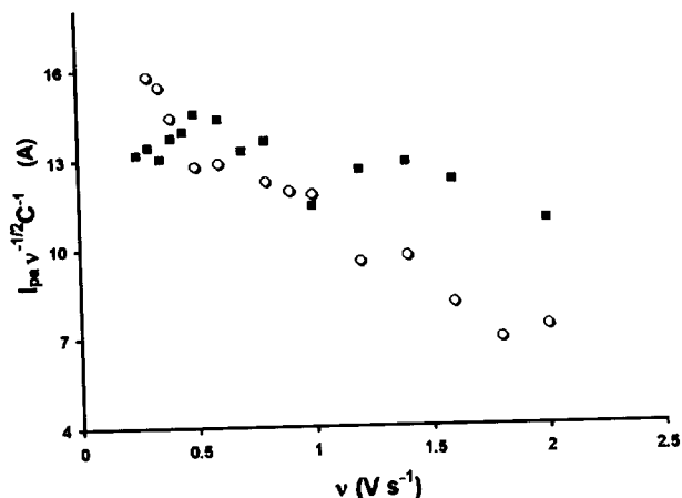
Figure 6. Variation of the voltammetric current function ( I_{pa} \nu^{-1/2} C^{-1} ) with scan rate potential ( \text{V s}^{-1} ) for both peaks of oligomer II: (■) peak I A ; (○) peak I IIA
