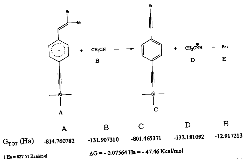
Figure 11. Oxidation reaction proposed for II . Gibbs free energies calculated at the B3LYP/LACVP** level of theory in the solution phase at standard temperature and pressure
