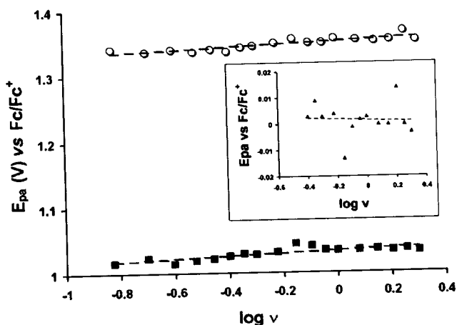
Figure 5. Variation of the potential of the oxidation peaks of 0.7 mm oligomer II with logarithm of the scan rate potential: (■) peak I A ; (○) peak I IIA ; (▲) Fc 0.7 mm at the onset. Slope values for the indicated regions are 19, 20 and 2 mV per decade, respectively
