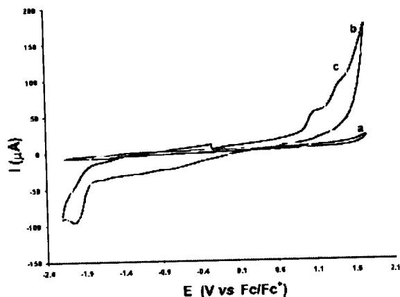
Figure 2. Typical cyclic voltammogram of oligomers II and IV (0.7 mm), obtained with a platinum microelectrode (0.033 cm 2 ) in 0.1 M TBAP in acetonitrile–dichloromethane (3:1). The potential scan was initiated from -0.25 V vs Fc/Fc + towards the positive direction (100 mV s -1 ). (a) Electro-analysis medium; (b) oligomer II present; (c) oligomer IV present
