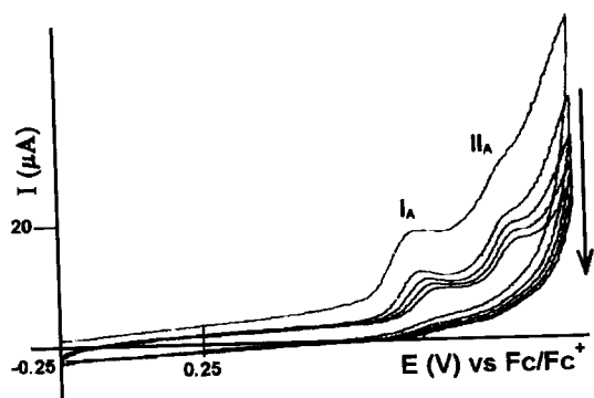
Figure 4. Five consecutive cyclic voltammograms of the anodic region of oligomer II (0.7 mm) obtained with a platinum microelectrode ( 0.033 \text{ cm}^2 ) in 0.1 M TBAP in acetonitrile–dichloromethane (3:1). The potential scan was initiated from -0.25 \text{ V vs Fc/Fc}^+ towards the positive direction ( 100 \text{ mV s}^{-1} )
