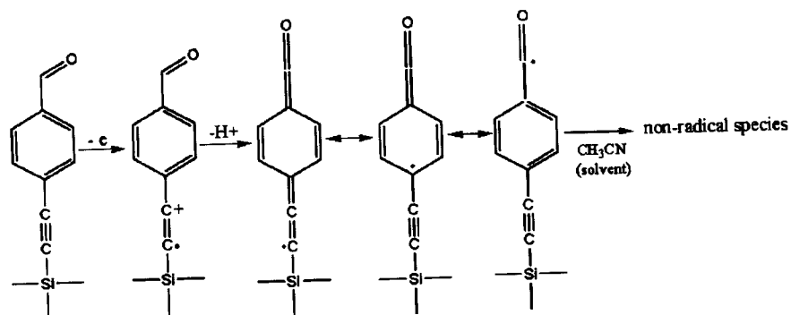
Figure 8. Resonant structures for cation-radical oligomer with formyl terminal groups
