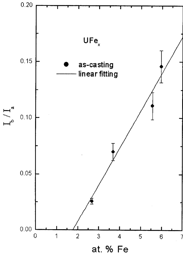
FIGURE 3. The ratio of intensities I_b/I_a for as-casting alloys at different at. % of Fe. The solid line is a linear fit.
