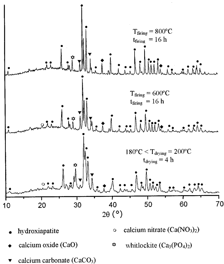
FIGURE 6. XRD of sample obtained by the Sol-gel process, after drying 4h, 180 < T < 200^{\circ}\text{C} (a); after calcinations during 16h at 600^{\circ}\text{C} (b); and at 800^{\circ}\text{C} (c).
