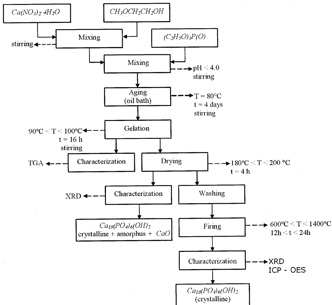
FIGURE 3. Flow chart for obtaining HA by the sol gel process.
