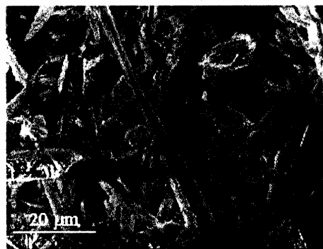
Fig. 10. SEM image of \text{Li}_2\text{SiO}_3 after a thermal treatment at 1400^\circ\text{C} for 4 h.
