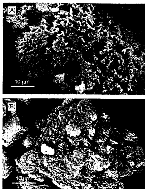
Fig. 2. SEM images of \text{Li}_2\text{SiO}_3 (A) and \text{Li}_4\text{SiO}_4 (B) powders.
