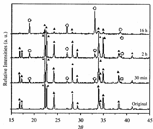
Fig. 4. XRD patterns of \text{Li}_4\text{SiO}_4 powders heat-treated at 1000 °C for different times. The labels correspond to (▲) \text{Li}_4\text{SiO}_4 and (○) to \text{Li}_2\text{SiO}_3 , respectively.
