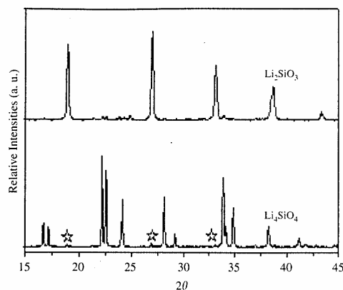
Fig. 1. Powder diffraction patterns of \text{Li}_2\text{SiO}_3 and \text{Li}_4\text{SiO}_4 powders after the syntheses processes. Peaks labelled with ☆ correspond to \text{Li}_2\text{SiO}_3 minor impurities in the \text{Li}_4\text{SiO}_4 sample.
