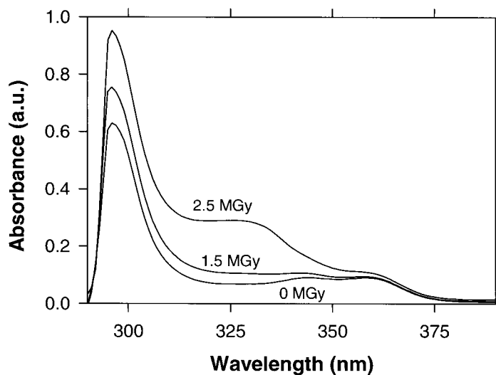
Figure 2. UV spectra of the starting and irradiated PBT.
