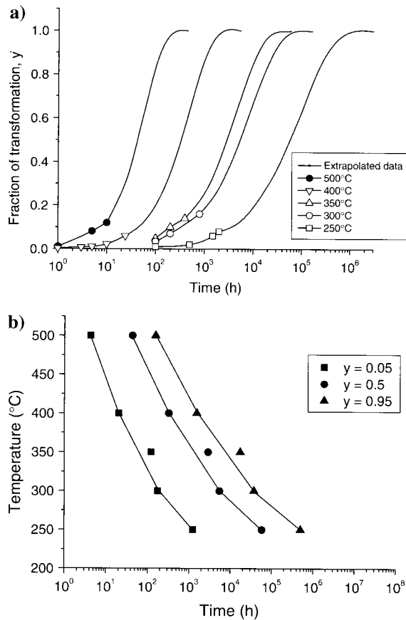
Fig. 8 (a) Avrami curves and (b) TTT curves obtained from results
