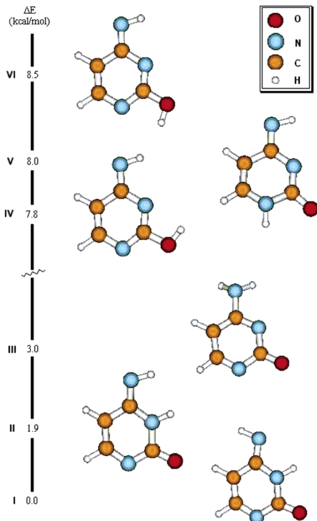
Figure 1. Optimized structures and relative energies (kcal/mol) of Cyē⁻ at the MP2/6-311+G(2d,p) level of theory.
