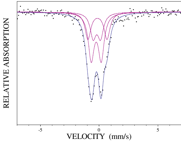
Fig. 9 Mössbauer spectrum of (\text{Ru}_{0.975}\text{Fe}_{0.025})\text{Sr}_2\text{GdCu}_2\text{O}_{8-\delta} at 25 K
