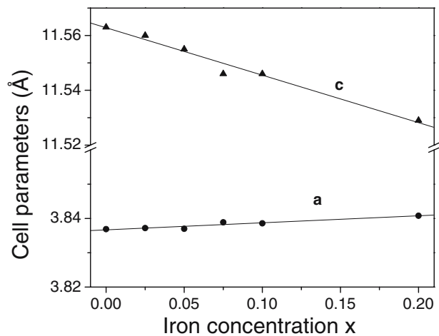
Fig. 3 Crystal lattice parameters as a function of Fe content x
