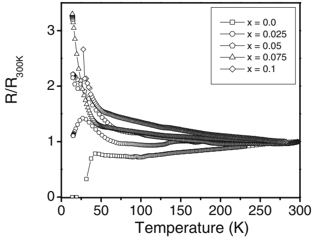
Fig. 4 Normalized resistance as a function of temperature of the \text{Ru}_{1-x}\text{Fe}_x\text{-1212} samples
