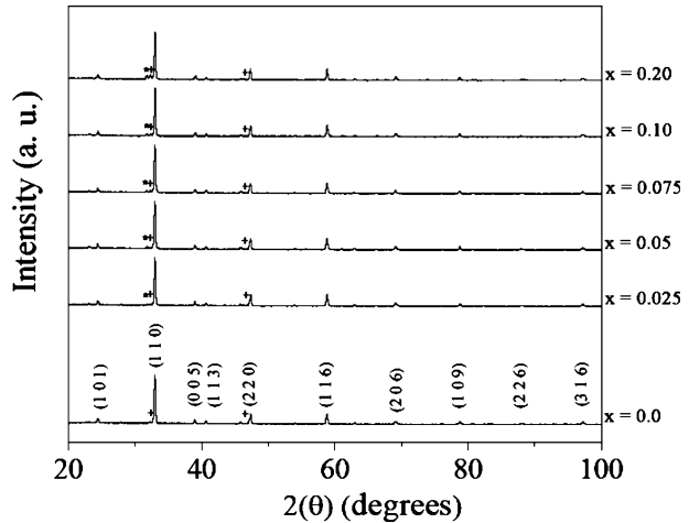
Fig. 1 X-ray diffraction patterns for the (\text{Ru}_{1-x}\text{Fe}_x)\text{Sr}_2\text{GdCu}_2\text{O}_8 samples. The symbols + and * point out peaks of \text{SrRuO}_3 or \text{Gd}_2\text{CuO}_4 and \text{Sr}_3(\text{Ru,Cu})\text{O}_7 impurity phases, respectively
