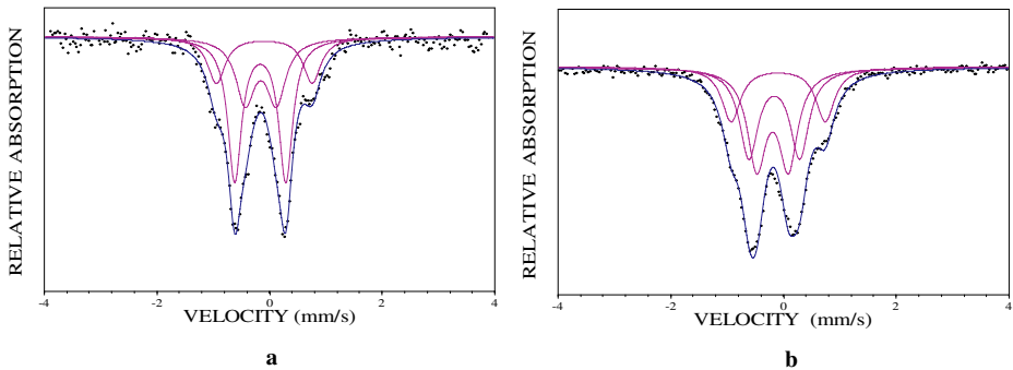
Fig. 5 Room temperature Mössbauer spectra of (\text{Ru}_{1-x}\text{Fe}_x)\text{Sr}_2\text{GdCu}_2\text{O}_8 a x=0.025 and b x=0.2
