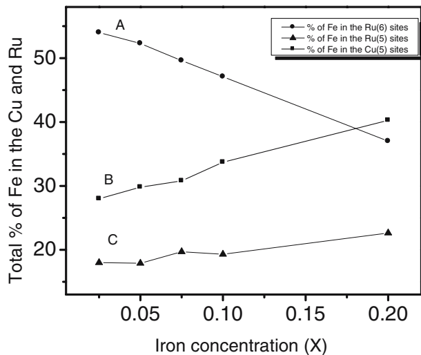
Fig. 6 Total Fe percent population in the different sites of the structure
