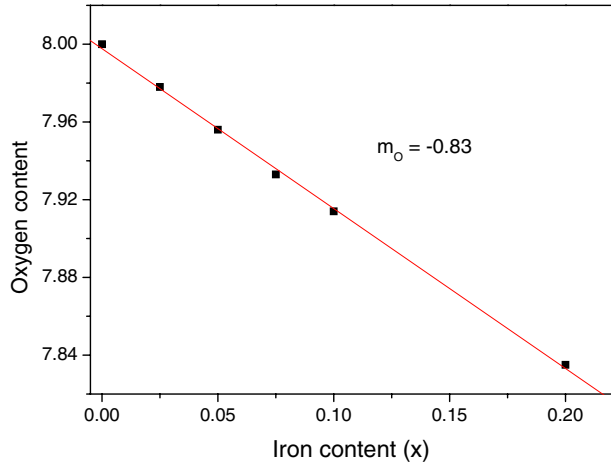
Fig. 7 Oxygen content as a function of iron concentration
