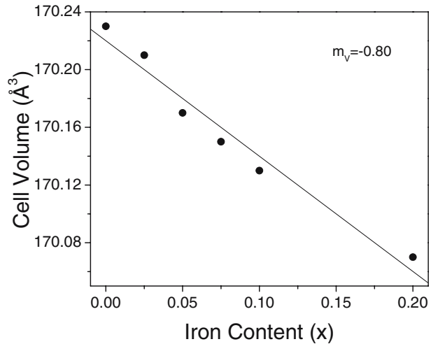
Fig. 8 Cell volume as a function of iron concentration x
