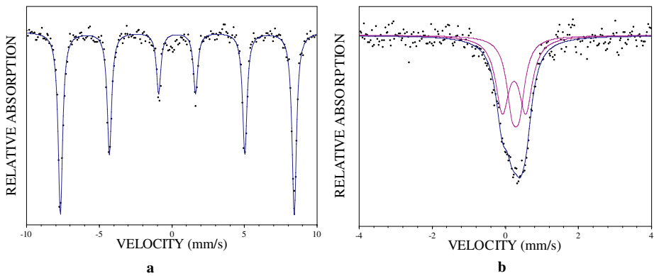
Fig. 10 Room temperature Mössbauer spectra of a \text{Gd}_2\text{Cu}_{0.95}\text{Fe}_{0.05}\text{O}_4 and b \text{SrRu}_{0.95}\text{Fe}_{0.05}\text{O}_3
