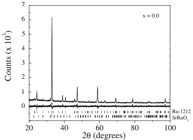
Fig. 2 Rietveld refinement of the X-ray diffraction pattern for the x=0.0 sample. Experimental spectrum (dots), calculated pattern (continuous line), their difference (middle line) and the calculated peak positions (bottom)
