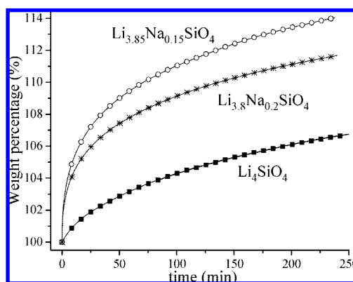
Figure 5. Isothermal analyses of Li 4-x Na x SiO 4 samples heat-treated at 500 °C into a flux of CO 2 .
