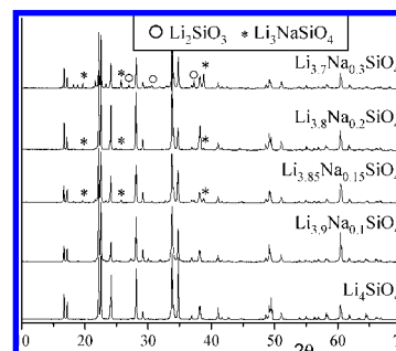
Figure 1. XRD patterns of different \text{Li}_{4-x}\text{Na}_x\text{SiO}_4 samples. Only the peaks corresponding to phases different than \text{Li}_4\text{SiO}_4 were labeled.
