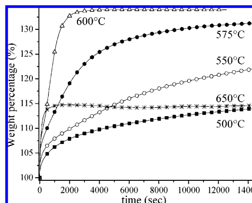
Figure 7. CO 2 absorption isothermal analyses of Li 3.85 Na 0.15 SiO 4 sample at different temperatures into a flux of CO 2 .
