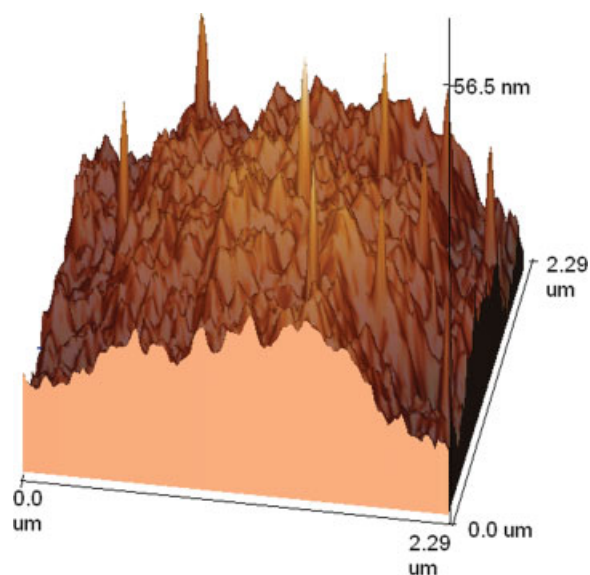
Figure 6 Surface image of poly(Bis-GMA/TEGDMA). Area 5.3 (\mu\text{m})^2 . [Color figure can be viewed in the online issue, which is available at www.interscience.wiley.com .]
