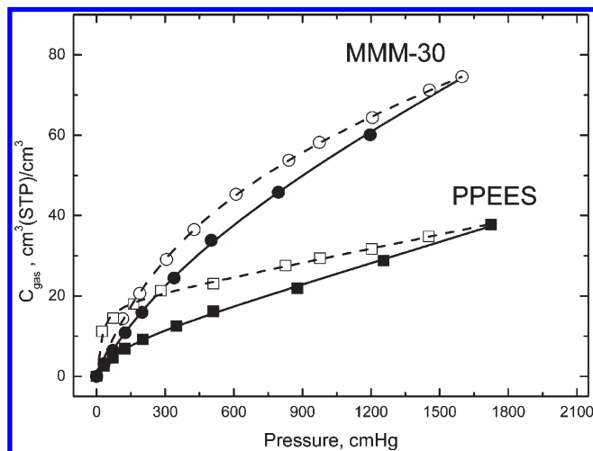
Figure 9. Variation of the concentration of sorbed (full symbols) and desorbed (open symbols) carbon dioxide with pressure for PPEES and MMM-30 at 303 K.
