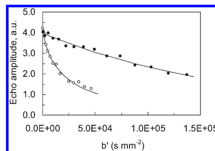
Figure 6. Plot of the peak intensity vs b' ( \text{s mm}^{-2} ) corresponding to ^{13}\text{C}]\text{O}_2 sorbed in polysulfone with 10% (w/w) ZIF-8 obtained with a diffusion time, \Delta , equal to (○) 10 ms and (●) 1500 ms. The duration, \delta , of the gradient pulse was kept constant to 2 ms, and the amplitude of the field gradient, g , in \text{G/cm} , was varied between 15 and 1760. For each data point, 48 scans were averaged with a TR of 15 s. The solid lines represent the best fits to the corresponding stretched exponential (eq 7).
