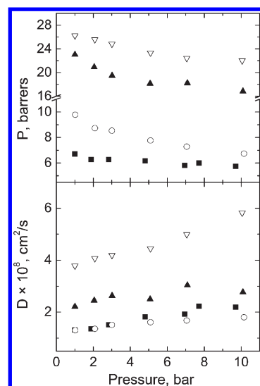
Figure 10. Variation of the permeability and diffusion coefficients of carbon dioxide with pressure, at 303 K, in membranes: (■) PPEES, (○) MMM-10, (▲) MMM-20, and (▽) MMM-30.
