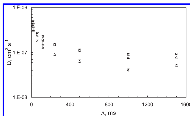
Figure 7. Variation of the apparent diffusion coefficient of ^{13}\text{C}]\text{O}_2 in the MMMs containing 10% (triangles), 20% (circles) and 30% (squares) w/w of ZIF-8, with the diffusion time \Delta . In all cases, the duration of the gradient pulse, \delta , was 2 ms.
