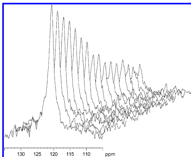
Figure 5. ^{13}\text{C} PFG NMR spectra corresponding to ^{13}\text{C}]\text{O}_2 sorbed in MMM-20 obtained with a diffusion time, \Delta , equal to 60 ms. The duration, \delta , of the gradient pulse was kept constant to 2 ms, and the amplitude of the field gradient, g , was incremented in 16 consecutive steps of 60 \text{ g cm}^{-1} from an initial value of 60 \text{ g cm}^{-1} .
