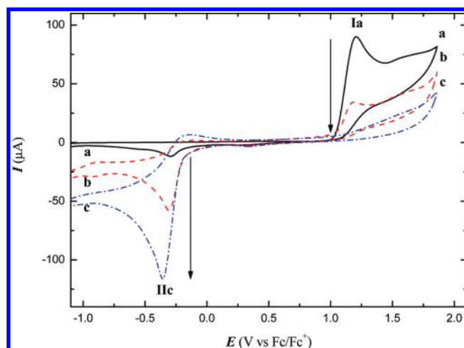
FIGURE 4. Cyclic voltammetry survey of the Py-GSATA (20 mM) electrolysis at 1.35 V vs \text{Fc}/\text{Fc}^+ in ACN and 0.1 M TBAP, using Pt electrodes in a divided cell: (a) 0, (b) 1.15, and (c) 2.3 F/mol.
