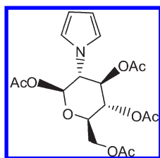
FIGURE 1. 1,3,4,6-Tetra- O -acetyl-2-(pyrro-1-yl)-2-deoxy- \beta -D-glucopyranose ( 1 , Py-GSATA).
