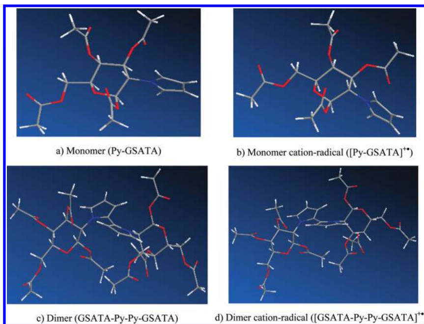
FIGURE 7. Optimized geometry of the Py-GSATA intermediates at B3LYP/6-31+G** level of theory. Dimer \sigma -dimer ([GSATA-(H)Py(H)-GSATA] 2+ ) and tetramer are depicted in Supporting Information (Figure S5).
