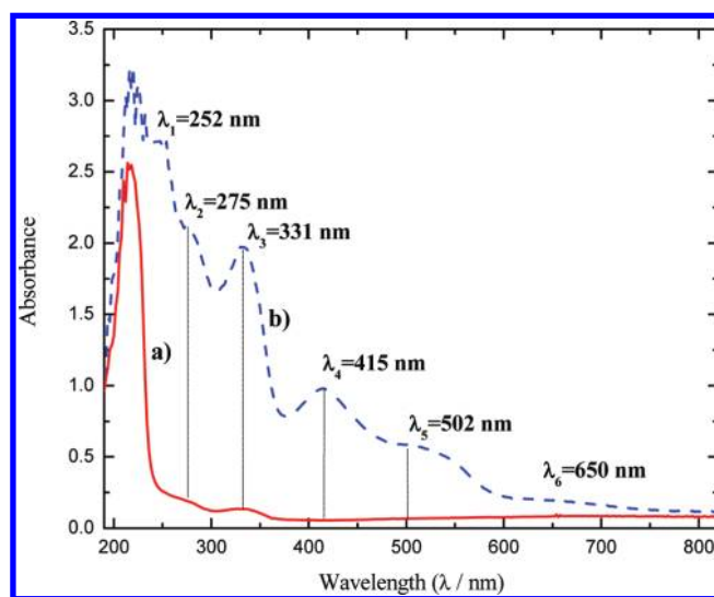
FIGURE 6. Initial (a) and final (b) UV-vis of the electrolysis at 1.42 V vs \text{Fc}/\text{Fc}^+ of a solution containing 0.1 M TBAP in ACN and 10 mM Py-GSATA. Cell volume 2 mL, using a Pt mesh as working electrode and in a separated compartment a copper mesh.
