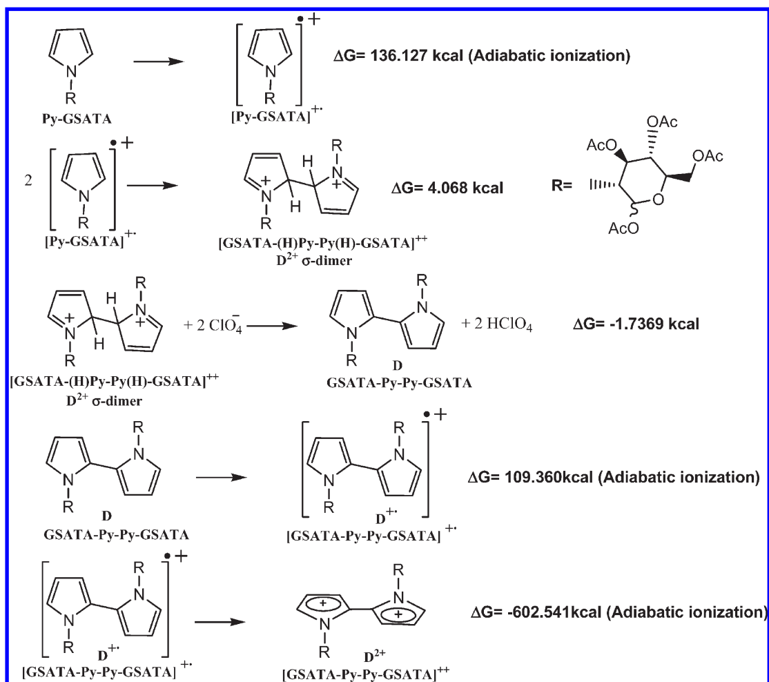
SCHEME 1. Thermochemical Analysis in Solution (ACN) of the Dimerization Process
