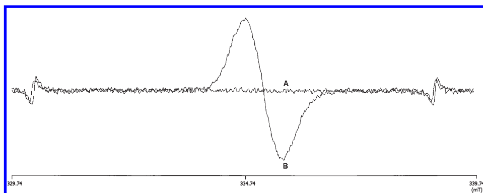
FIGURE 5. ESR spectra of (A) solution containing 0.1 M TBAP in ACN and 20 mM Py-GSATA (corresponds to Figure 5a) and (B) same solution analyzed after total electrolysis at 1.35 V vs \text{Fc}/\text{Fc}^+ (2.3 F/mol; corresponds to Figure 5c). Lateral ESR signals correspond to the internal standard \text{MnO} .
