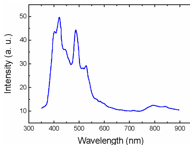
FIGURE 6. Spectrum of photoluminescence of \gamma -Fe 2 O 3 /ZnO composite particles under 358 nm excitation.
