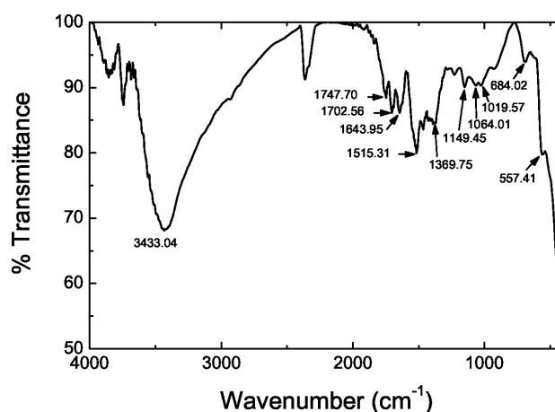
FIGURE 5. FT IR spectrum of \gamma -Fe 2 O 3 /ZnO composite particles.
