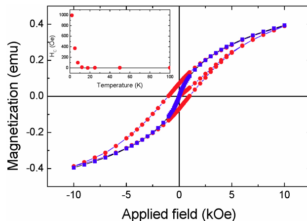
FIGURE 8. Magnetization as a function of applied magnetic field of a sample of \gamma -Fe 2 O 3 /ZnO composite, the curves were measured at 2 K (circles) and 12 K (squares). Note that the curve measured at 12 K does not show hysteresis. The inset shows the coercive field as a function of temperature.
