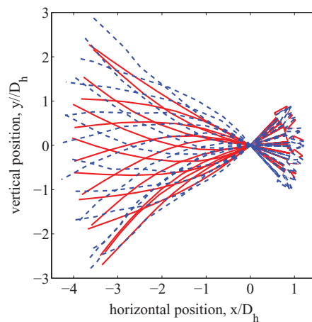
FIG. 8. Superimposed shapes of the flexible tail at different instants throughout the oscillation cycle. The solid (red) and dashed (blue) lines display the tail shape for the Newtonian (N2) and Boger (B2) fluids, respectively. These measurements correspond to the data shown in Fig. 3.
