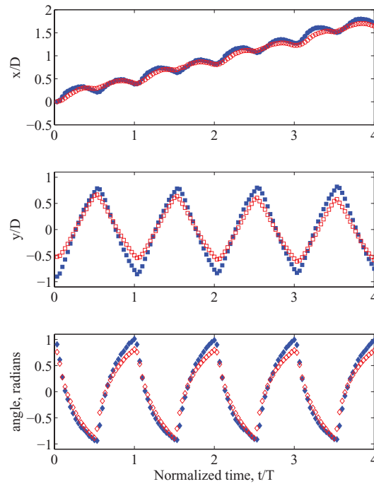
FIG. 3. Position of the head along ( \circ ) and across ( \square ) the swimming direction as well as head angle ( \diamond ); filled symbols (blue) show results for the Boger (B2) fluid while empty symbols (red) are for the Newtonian (N2) fluid.
