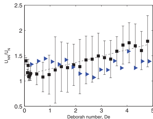
FIG. 6. Ratio of non-Newtonian ( U_{NN} ) to Newtonian ( U_N ) swimming speeds, U_{NN}/U_N , as a function of the Deborah number, De . ■ (black): fluids N2 and B2; ► (blue): fluids N1 and B1. The dashed line is a linear fit to the data for all fluids.
