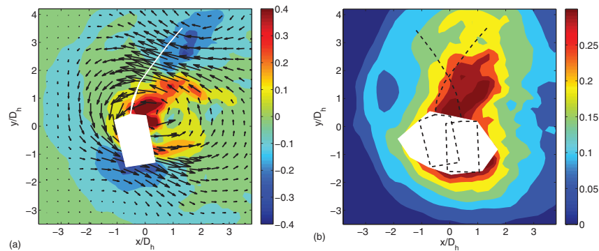
FIG. 7. PIV results for the flow field around the swimmer with a two-dimensional tail in fluid B2. (a) Vorticity (colors) and velocity (arrows) fields; (b) cycle-averaged magnitude, |\mathbf{D}| , of the rate-of-strain tensor, \mathbf{D} . Vorticity and rate-of-strain fields are normalized by the oscillation frequency, \omega . The white regions show the position of the swimmer at different instants throughout the cycle.
