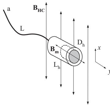
FIG. 1. Sketch of the magnetic swimmer with flexible tail. See text for notation.
