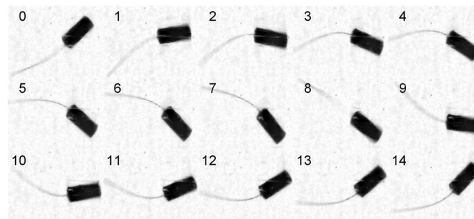
FIG. 2. Image sequence of a swimming cycle at frequency \omega = 1 Hz in the Boger fluid (B2); time step between each image, \Delta t = 66.6 ms.
