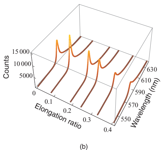
FIG. 5. (a) Output energy and FWHM as function of pump energy for the bovine pericardium sample. (b) Evolution of the random laser spectrum from the bovine pericardium during the elongation test.
