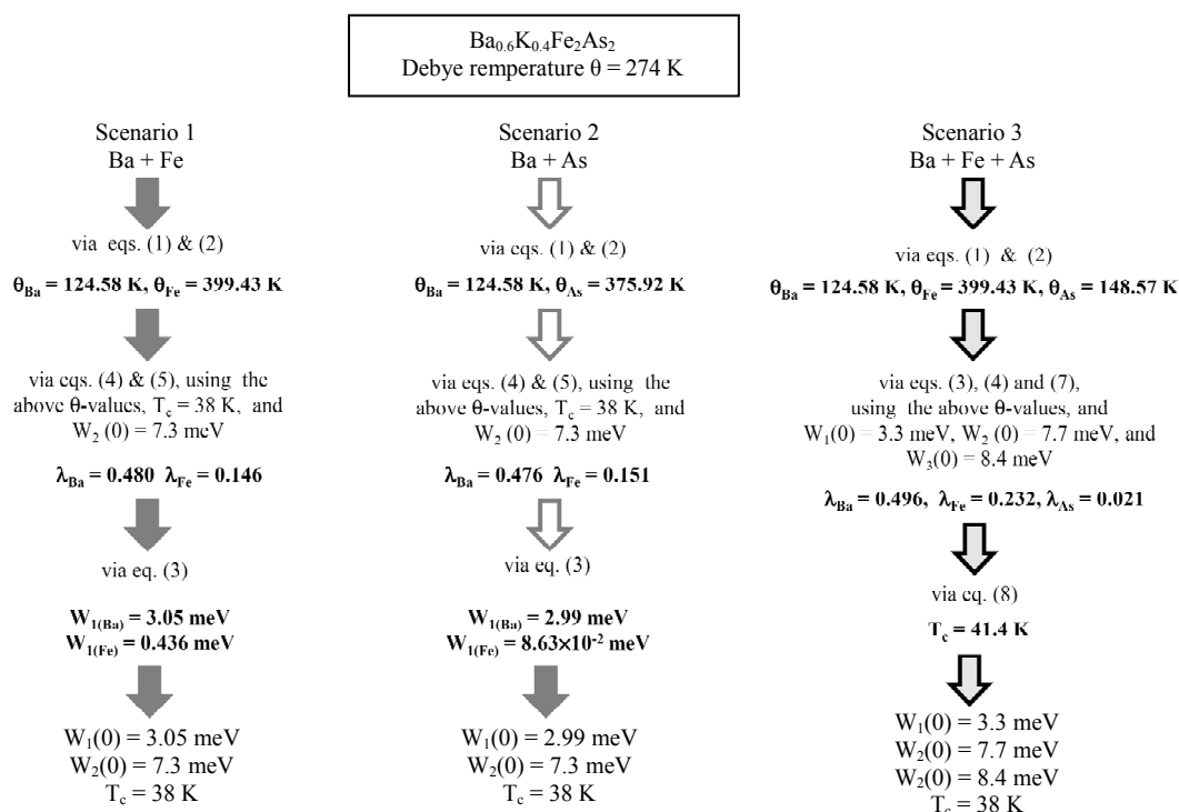
Figure 1. Schematic diagram giving the best-case values for the T_c and the gap-values led to by GBCSEs for Ba_{0.6}K_{0.4}Fe_2As_2 based on its characterization via 2- and 3-gap scenarios.
