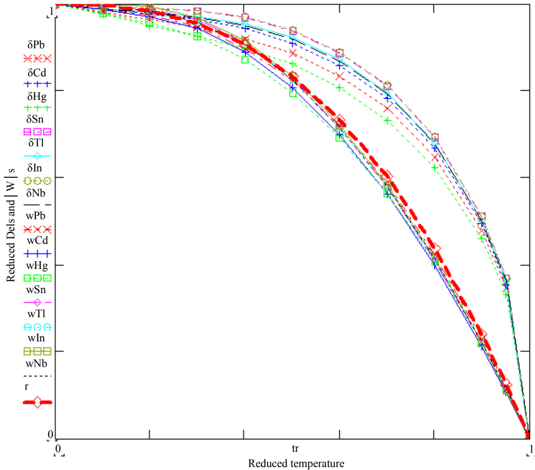
Figure 2. Plots of \Delta(T)/\Delta_0 obtained via (2) with variable \lambda given in (11), and of |W(T)|/|W_0| obtained via (4) with \lambda given in (12). The upper cluster of curves corresponds to \Delta(T)/\Delta_0 , and the lower to |W(T)|/|W_0| . The thick dashed curve corresponds to n_s = 1 - t^{2.6} .
