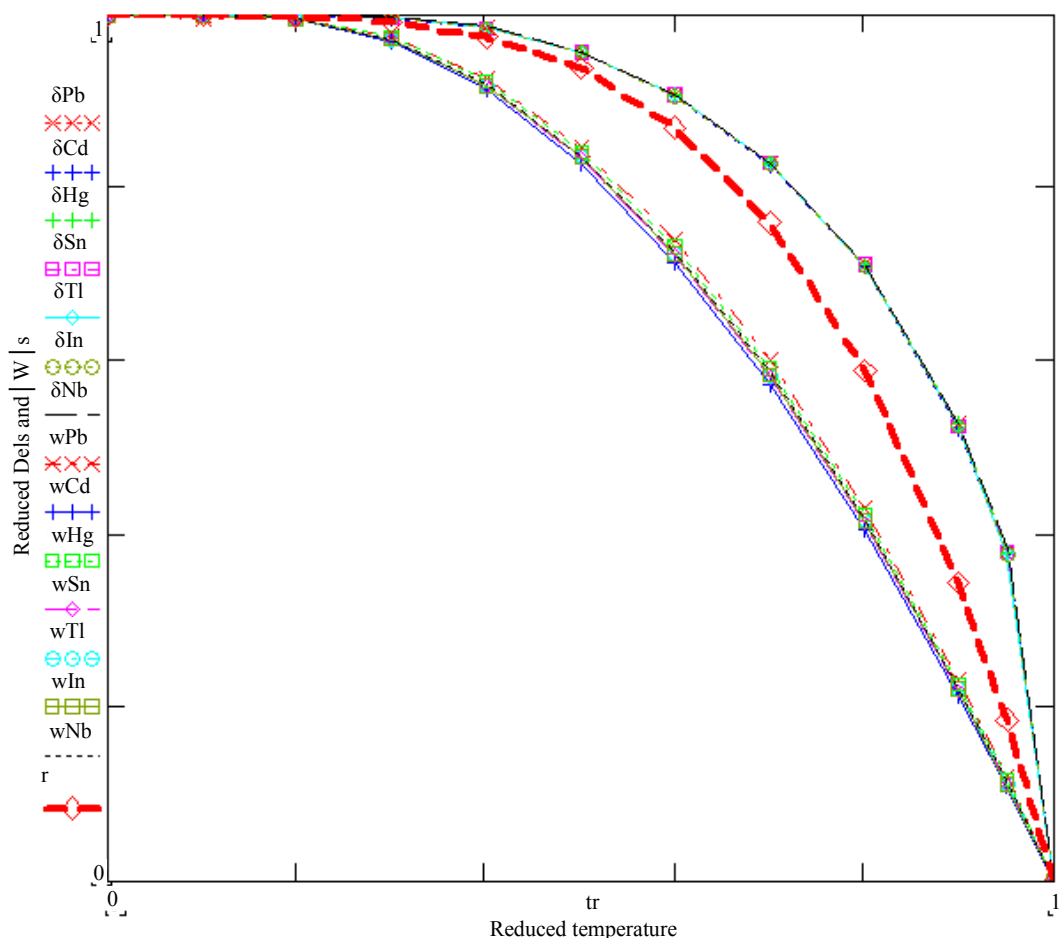
Figure 1. Plots of \Delta(T)/\Delta_0 obtained via (2), and of |W(T)|/|W_0| obtained via (4). \lambda in each case is taken to be \lambda(T_c) as given in Table 1. The upper cluster of curves corresponds to \Delta(T)/\Delta_0 , and the lower to |W(T)|/|W_0| . The thick dashed curve between the two clusters corresponds to n_s = 1 - t^4 , see (9).
