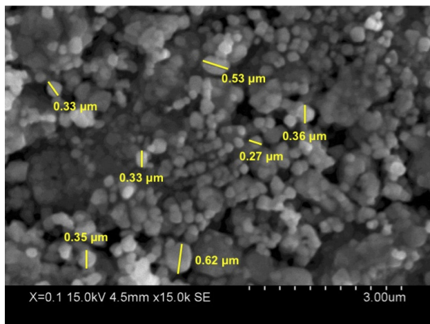
FIGURE 2. SEM of the \text{Er}_{1.90}\text{Sr}_{0.10}\text{Ru}_2\text{O}_{6.95} sample.
