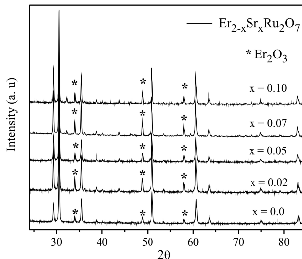
FIGURE 1. XDR Patterns evolution of (\text{Er}_{2-x}\text{Sr}_x)\text{Ru}_2\text{O}_7 system, with x = 0.0, 0.02, 0.05, 0.07 , and 0.10 .
