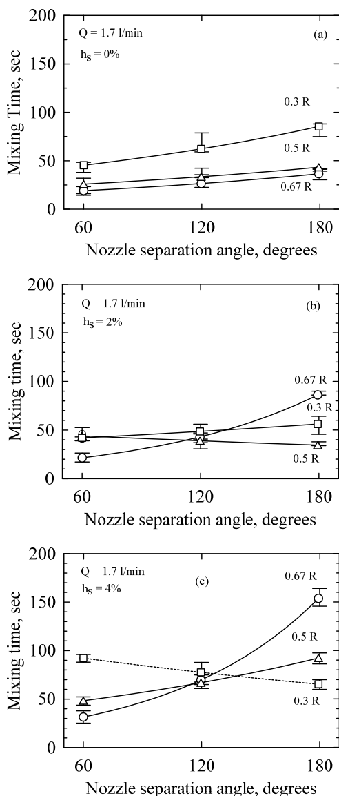
Fig. 6. Effect of nozzle separation angle on mixing time at different nozzle radial positions, for a gas flow rate of 1.7 Nl/min and different slag thicknesses; (a) 0%, (b) 2% (c) 4%.
